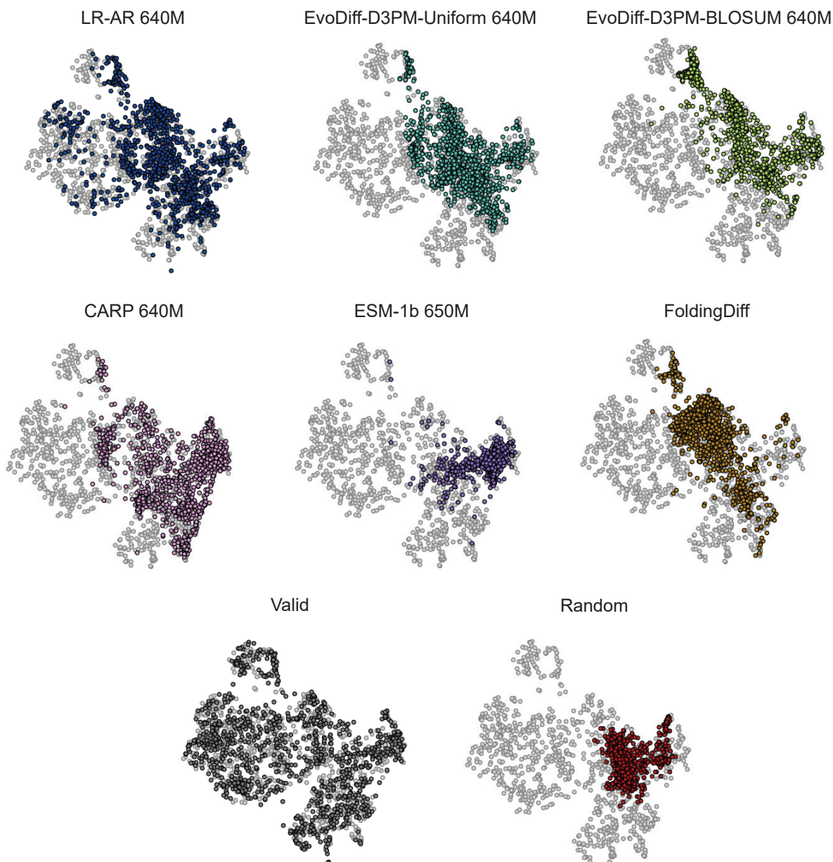
Figure S6: Coverage of sequence and functional space for generated distributions from 640M parameter EvoDiff sequence models and baselines. UMAP of ProtT5 embeddings, annotated with FPD, of natural sequences from test set (grey, n=1000 ) and of generated sequences from EvoDiff 640M parameter models and baselines (various colors, n=1000 ). A visualization of sequences from the validation set (dark grey, n=1000 ) is included for reference. The visualization for the 640M OADM model is excluded due to inclusion in Fig. 3A.
