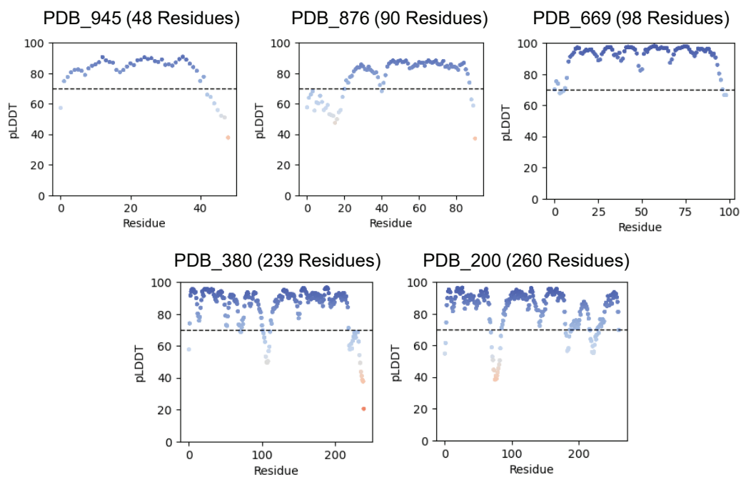
Figure S4: Per-residue pLDDT for representative proteins generated by EvoDiff-Seq. pLDDT scores computed based on the OmegaFold predicted structures, for individual residues in representative high-fidelity generations from EvoDiff-Seq (Fig. 2E). Points are colored by pLDDT (0-100, red to blue).
