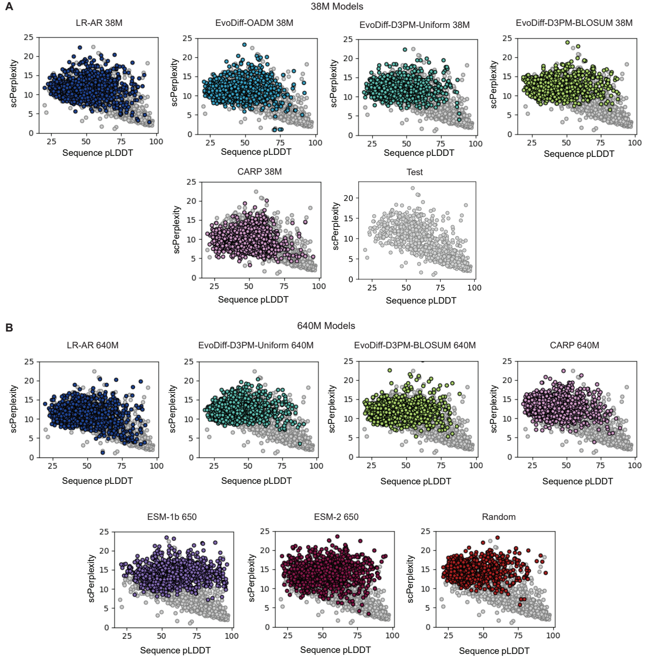
Figure S3: Sequence pLDDT versus self-consistency perplexity for EvoDiff sequence models. (A-B) Results for sequences from 38M parameter EvoDiff, baseline models, and test data plotted alone (A), and 640M parameter EvoDiff and baseline models (B) (various colors, n=1000 ), except for EvoDiff-OADM-640M (EvoDiff-Seq, shown in Fig. 2C), relative to sequences from the test set (grey, n=1000 ). The self-consistency perplexity (ESM-IF Perplexity) is computed using sequences inverse-folded by ESM-IF.
