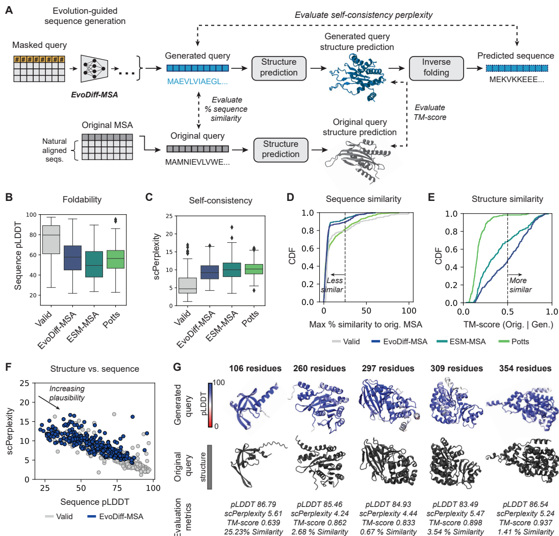
Figure S8: EvoDiff-MSA enables evolution-guided sequence generation. (A) A new sequence is generated from EvoDiff-MSA via diffusion over only the query component. Generations are evaluated for diversity and self-consistency and for the quality and consistency of their predicted structures. (B-E) Distributions of pLDDT (B), scPerplexity (C), sequence similarity (D; dashed line at 25%), and TM-score (E; dashed line at 0.5) for sequences from the validation set, EvoDiff-MSA, ESM-MSA, and a Potts model ( n=250 sequences per model; box plots show median and interquartile range). (F) Sequence pLDDT versus scPerplexity for sequences from the validation set (grey, n=250 ) and EvoDiff-MSA (blue, n=250 ). (G) Predicted structures and metrics for structurally plausible generations from EvoDiff-MSA.
