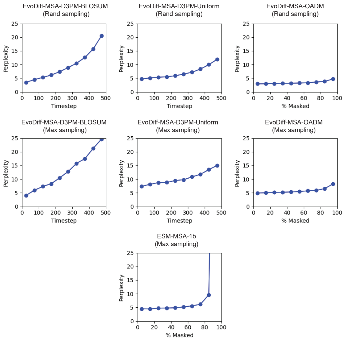
Figure S9: Perplexity as a function of corruption step for EvoDiff MSA models. Test-set MSA perplexities at sampled intervals of the degree of corruption, specifically the diffusion timestep for D3PM models and the fraction of masked residues for OADM and ESM models. The test-set evaluated for each model was sampled using the same sampling scheme assigned during training. Intervals reflect evenly spaced windows of 50 timesteps for D3PM models or 10% masking for masked models.
