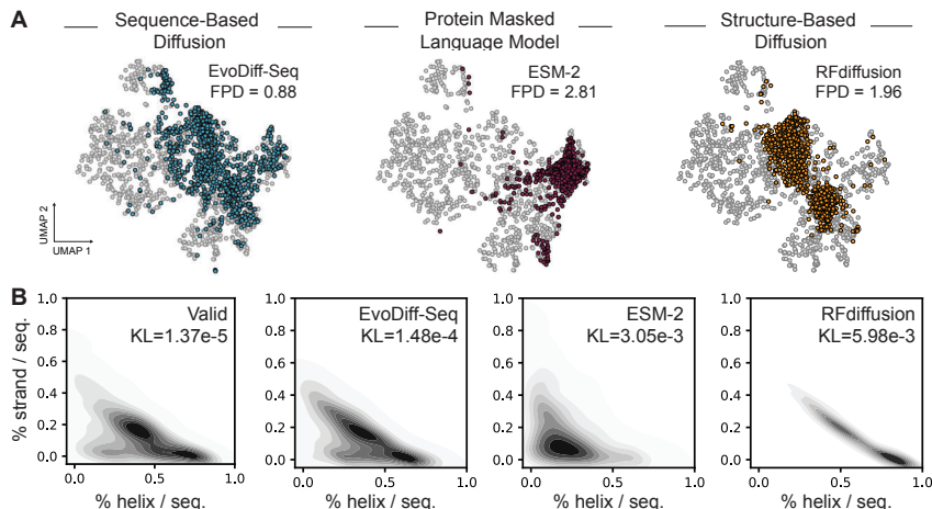
Figure 3: Generated protein sequences capture natural distributions of protein functional and structural features. (A) UMAP of ProtT5 embeddings, with Fréchet ProtT5 distance (FPD), of natural sequences from the test set (grey, n=1000 ) and of generated sequences from EvoDiff-Seq (blue, n=1000 ) and ESM-2 (red, n=1000 ), and inferred sequences inverse-folded from structures from RFdiffusion (orange, n=1000 ). (B) Distributions of structural features from DSSP 3-state predictions of generations ( n=1000 ), and their Kullback-Leibler (KL) divergence relative to the test set.
