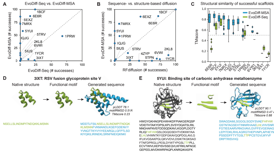
Figure 4: Scaffolding functional motifs without explicit structural information. (A) Successes from n=100 trials for EvoDiff-Seq (x-axis) versus EvoDiff-MSA (y-axis) across scaffolding problems in which at least one method succeeds. (B) Comparison of sequence-based scaffolding via EvoDiff-MSA (y-axis) vs. structure-based scaffolding via RFdiffusion (x-axis) across problems in which at least one method succeeds ( n=100 trials per problem). (C) Distributions of TM-scores of successfully generated scaffolds from EvoDiff models relative to the true structures (dashed line at 0.5). (D-E) Generated sequences, predicted structures, and metrics for scaffolding examples from EvoDiff-Seq (D) and EvoDiff-MSA (E). Motif: green, original scaffold: black, generated scaffold: blue.
