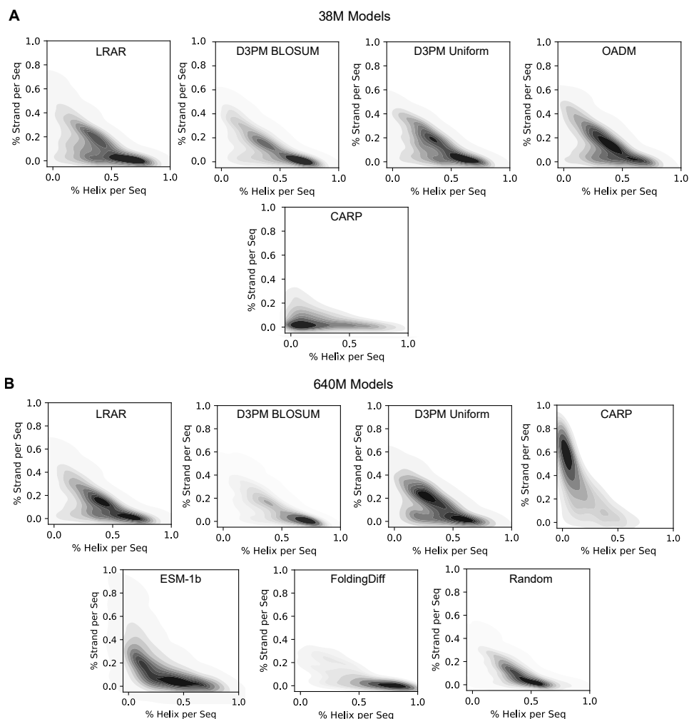
Figure S7: Structural features in generated sequences from all sequence models. (A-B) Multi-variate distributions of helix and strand features in sequences from 38M (A) and 640M (B) parameter models, and baselines based on DSSP 3-state predictions and annotated with the KL divergence relative to the test set ( n=1000 samples from each model). In (B), the distribution for the 640M OADM model is excluded (see Fig. 3B); the distribution for random sequences ( n=1000 ) is provided as reference.
