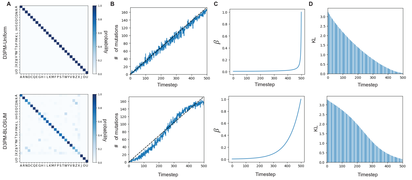
Figure S14: Details of EvoDiff-D3PM corruption schemes. The top and bottom rows correspond to EvoDiff-D3PM-Uniform and EvoDiff-D3PM-BLOSUM, respectively. (A) Visualization of EvoDiff-D3PM transition matrices. (B) Evolution of the number of mutations accrued as a function of the diffusion timestep t for a sample input. (C) Evolution of \beta as a function of the diffusion timestep t . (D) Evolution of D_{KL} [q(x_t|x_0)||p(x_T)] as a function of the diffusion timestep t , indicating convergence to a uniform stationary distribution at t = 500 as D_{KL} approaches zero.
