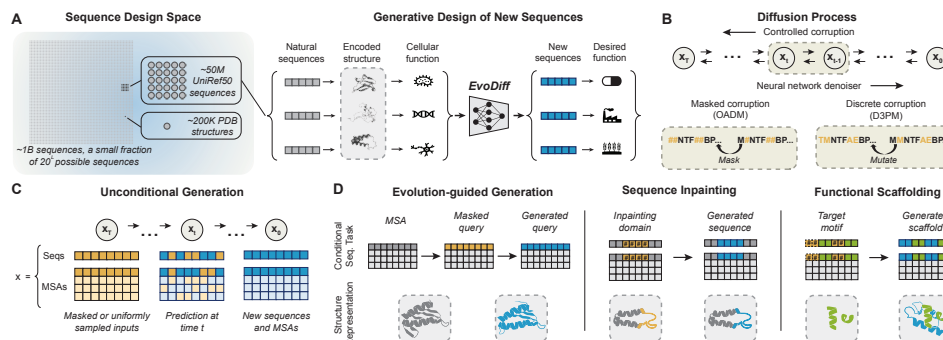
Figure 1: Protein sequence generation with evolutionary diffusion. (A) (Left) Evolution has sampled a tiny fraction of possible protein sequences. Experimental structures have been determined for even fewer proteins. (Right) EvoDiff is a generative discrete diffusion model trained on natural protein sequences. (B) Discrete diffusion models consist of controlled corruption and learned denoising processes. In masked corruption, input tokens are masked in an order-agnostic fashion (bottom, left). In discrete corruption, inputs are corrupted via a Markov process controlled by a transition matrix of amino acid mutation frequencies (bottom, right). (C) EvoDiff enables unconditional generation of protein sequences or MSAs. (D) Controllable design with EvoDiff, by conditioning on evolutionary information encoded in MSAs (left); inpainting functional domains (middle); or scaffolding (right).
