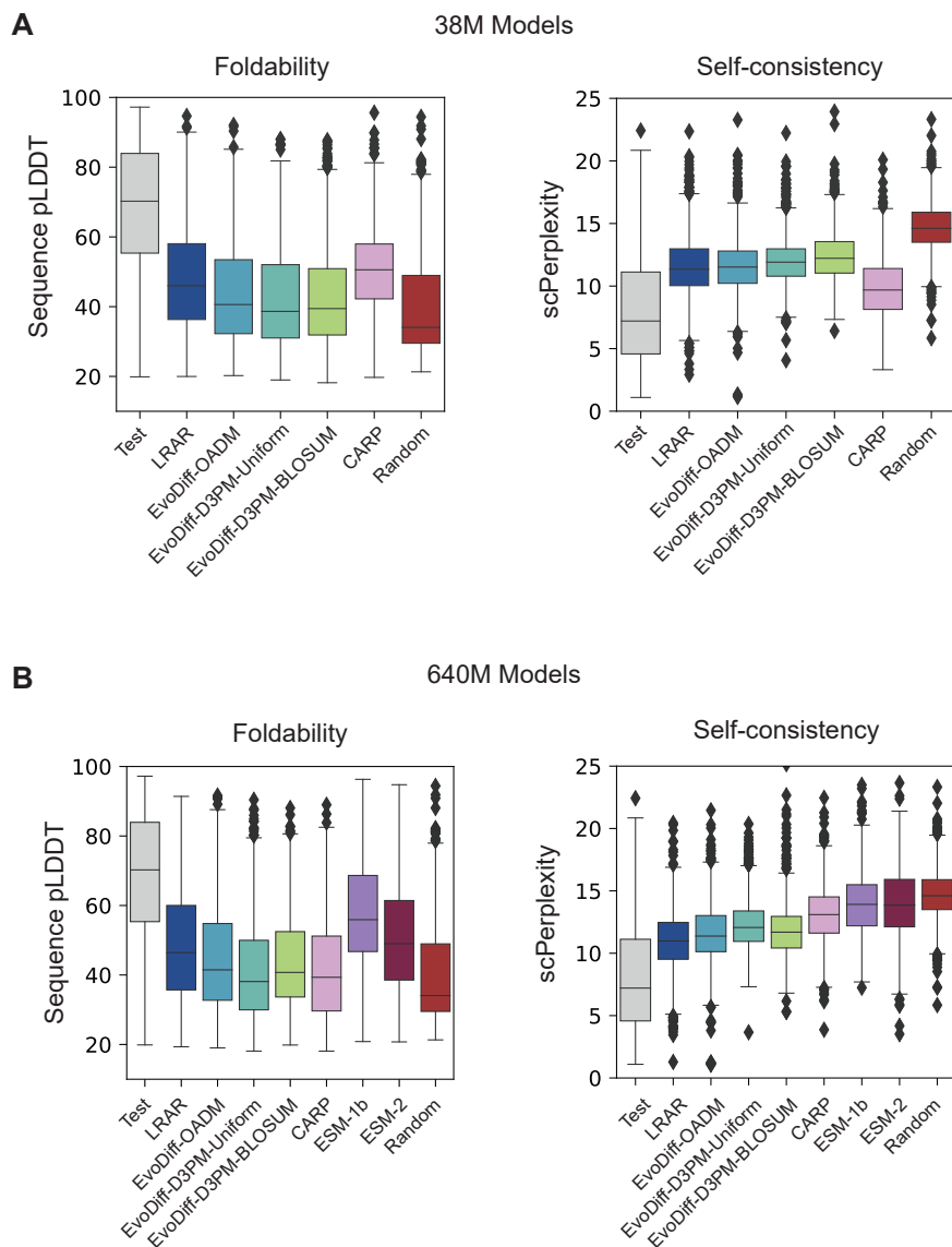
Figure S2: Summary statistics for structural plausibility metrics for sequence models. (A-B) Distribution of pLDDT and scPerplexity metrics for sequences from the test set, 38M parameter EvoDiff and baseline models (A), and 640M parameter EvoDiff and baseline models (B) (n=1000 sequences per model). Test and Random baselines are reproduced in (A) and (B) for reference.
