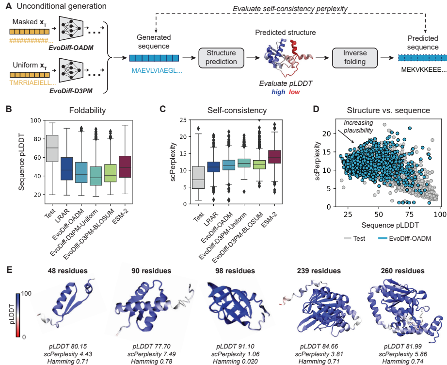
Figure 2: EvoDiff generates realistic and structurally-plausible protein sequences. (A) Workflow for evaluating sequences generated by EvoDiff sequence models. (B-C) Distributions of foldability, measured by sequence pLDDT of predicted structures (B), and self-consistency, measured by scPerplexity (C), for sequences from the test set, EvoDiff models, and baselines ( n=1000 sequences per model). (D) Sequence pLDDT vs. scPerplexity for sequences from the test set (grey, n=1000 ) and the 640M-parameter OADM model EvoDiff-Seq (blue, n=1000 ). (E) Predicted structures and metrics for select structurally plausible generations from EvoDiff-Seq, the 640M-parameter OADM model.
